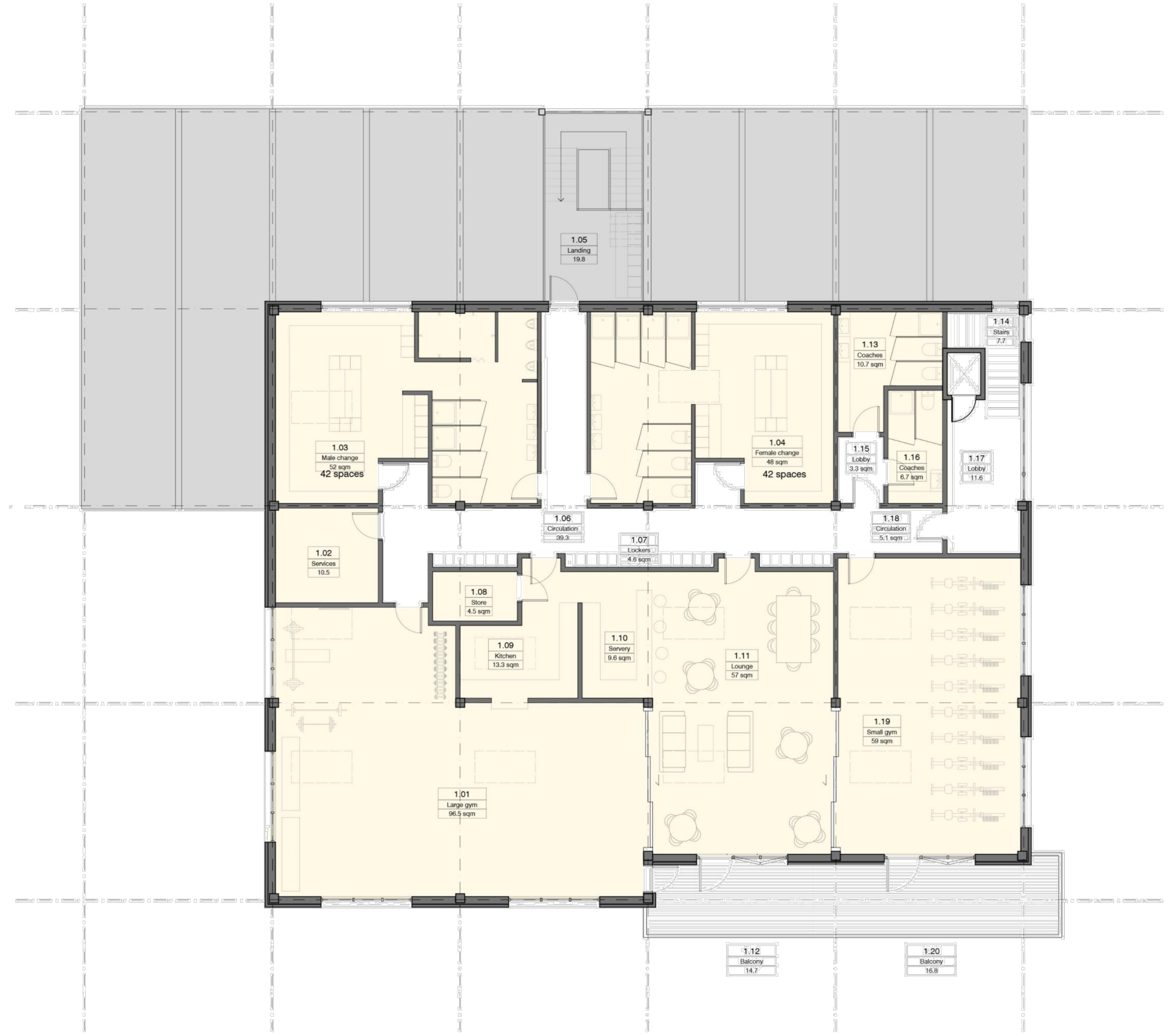
2 First Floor Plan 1:100
